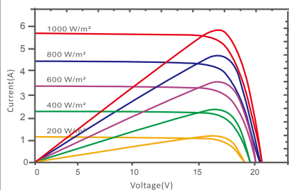
I-V characteristics at different irradiancies
